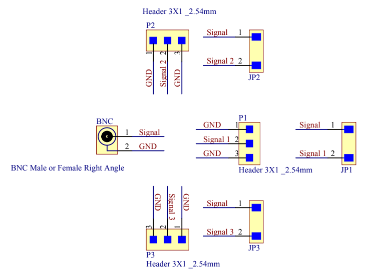
BNC-BO-V1A Schematic Diagram
