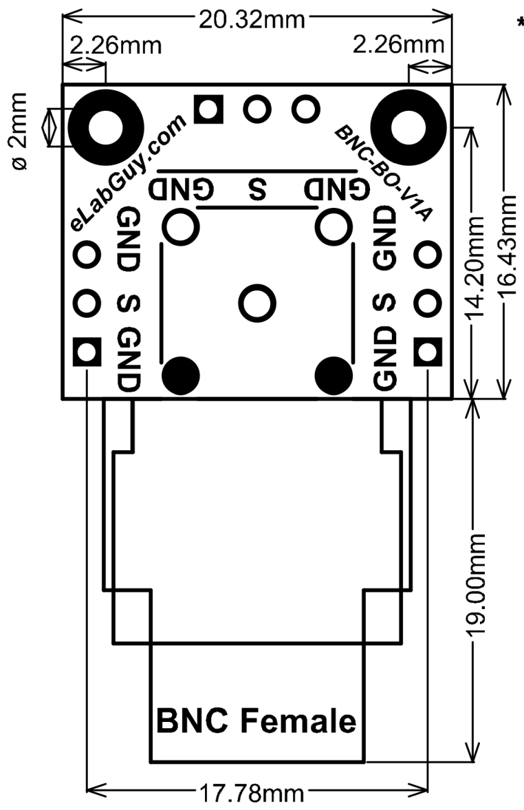
BNC-BO-V1A PCB outline Drawing
